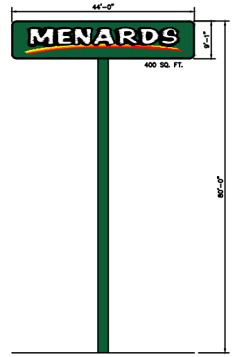
PYLON SIGN
